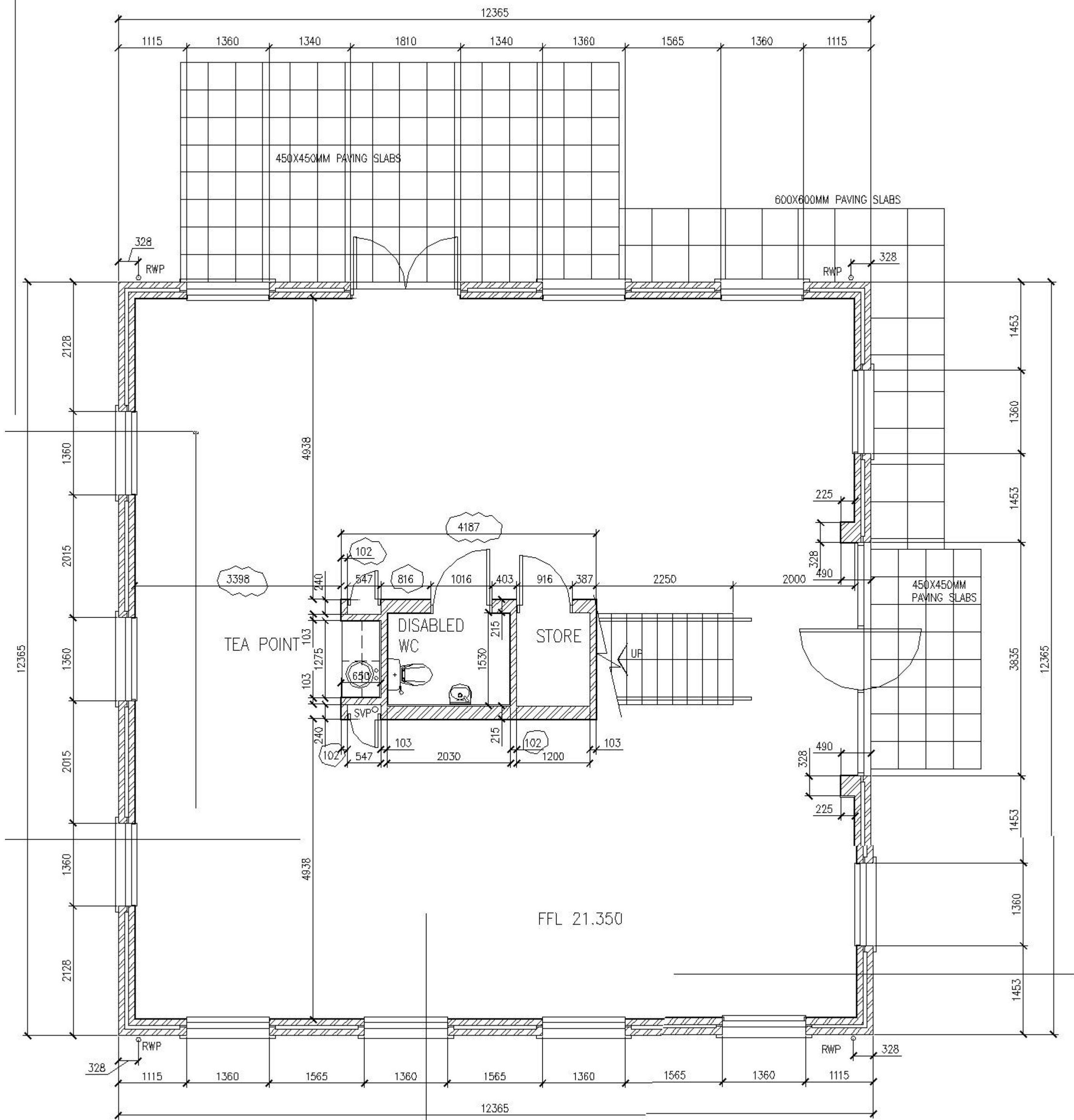
UNIT D GROUND FLOOR PLAN Scale 1:50
