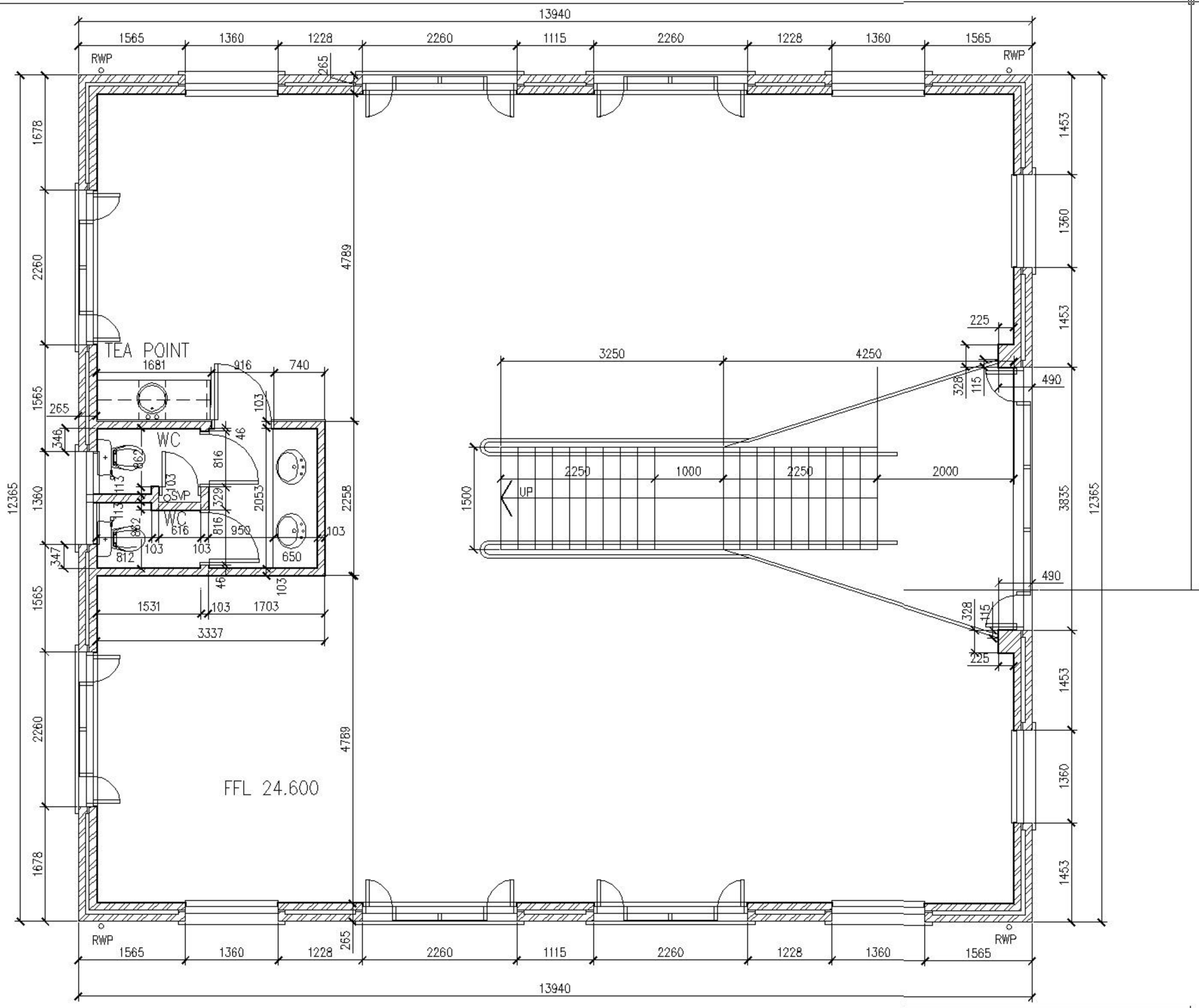
UNIT C FIRST FLOOR PLAN Scale 1:50
